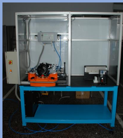
STAND FOR TIGHTNESS CONTROL AIR-AIR FOR DISTRIBUTING FRAME WITH INJECTION UNIT
