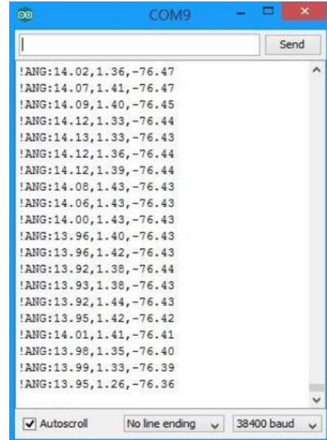
Figure 15: Output data when the remote control had an inclination of 15 degrees with respect to a horizontal plane about the roll axis
