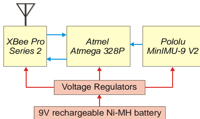
Figure 6: Block diagram of the developed remote control
