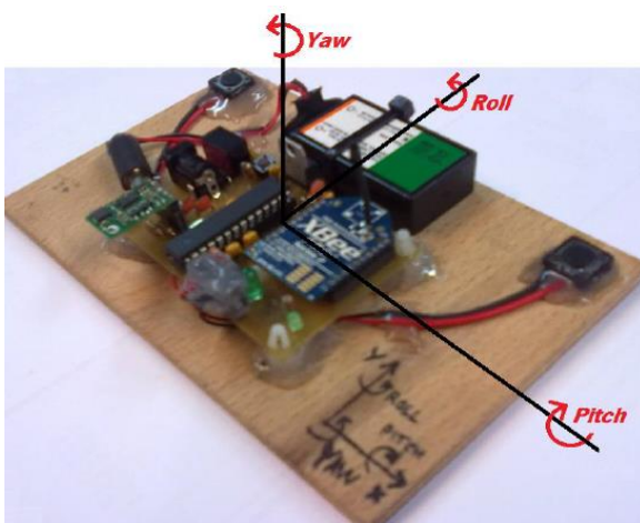
Figure 14: Prototype of the remote control, evidencing the hardware and the referential considered.
