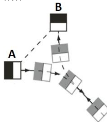
Figure 1: Trajectory described by a mobile platform with the Ackermann steering system in order to move from a point A to a point B [2].
