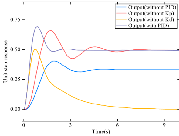
Figure 20: Step Response Diagrams Before and After Third-Order System Correction
